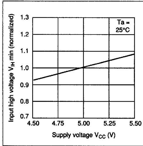
Input High Voltage vs. Supply Voltage
