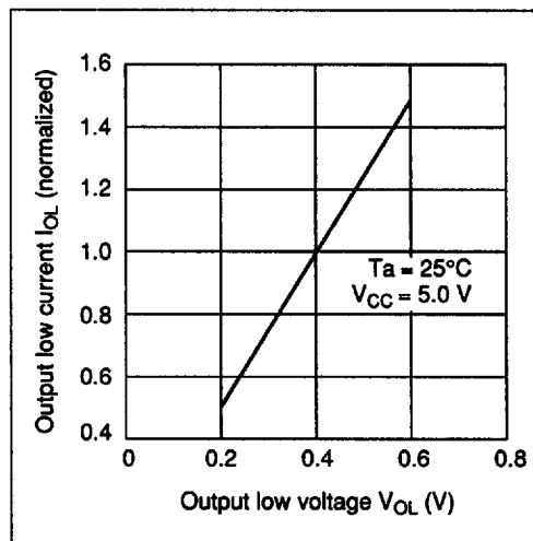
Output Low Current vs. Output Low Voltage
